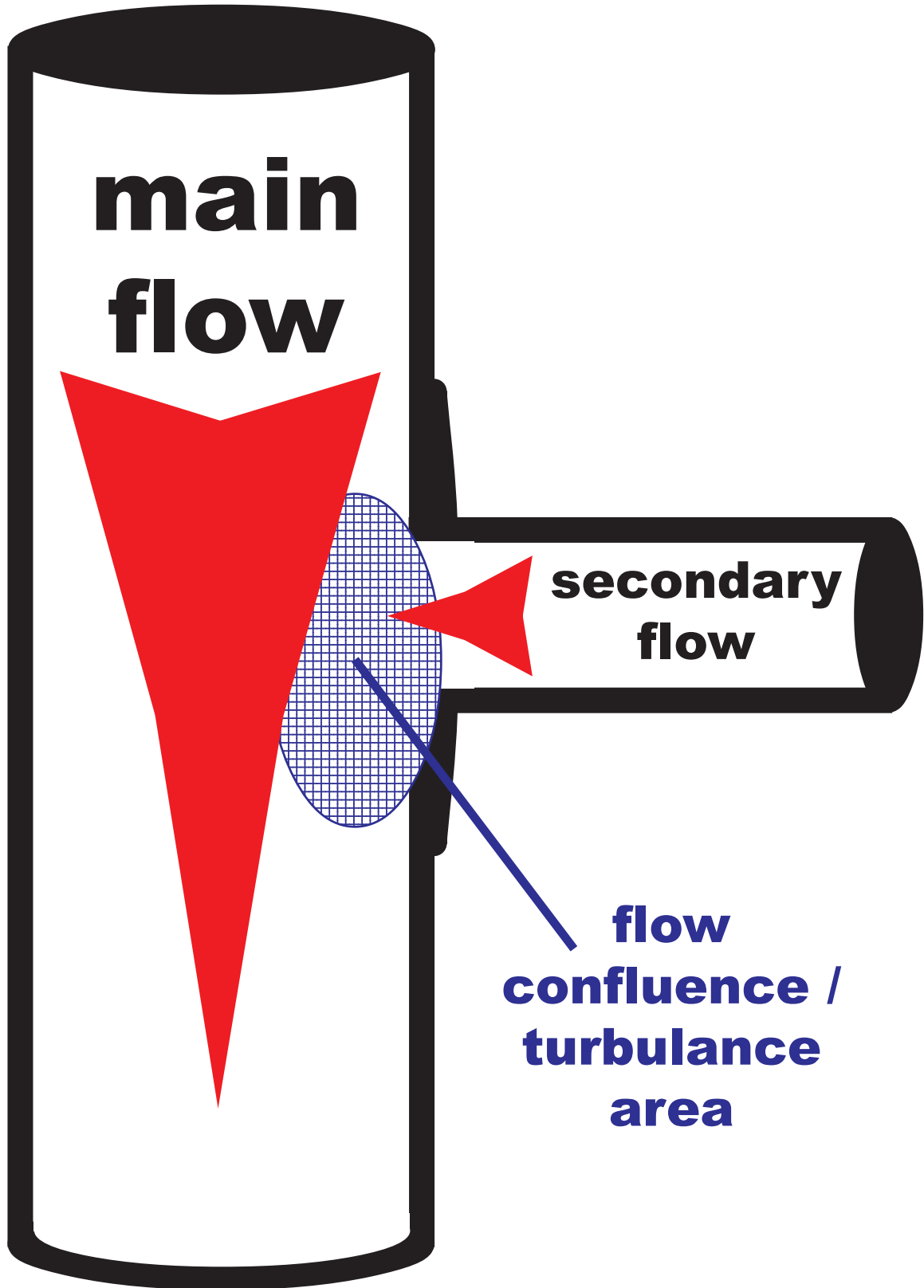
Figure 1: A pipe model of material flow and a confluence of two converging flow pathways.
